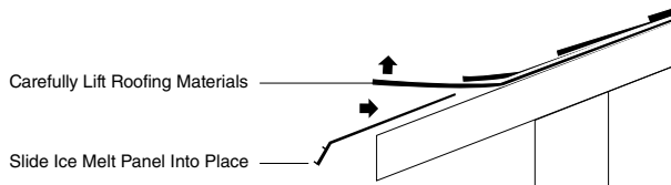
Detail 2. Installing the Ice Melt Panel on an existing roof.
