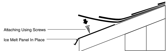
Detail 5. Screw the Ice Melt Panel into place.
