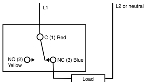
Detail 2 A19AN-1C Wiring Diagram for heating mode (opens or rise). Wire Common (1) to NC (3)
