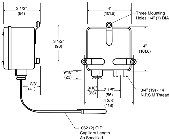
Detail 1 A19ANC-1C enclosure dimensions shown in inches (mm)
