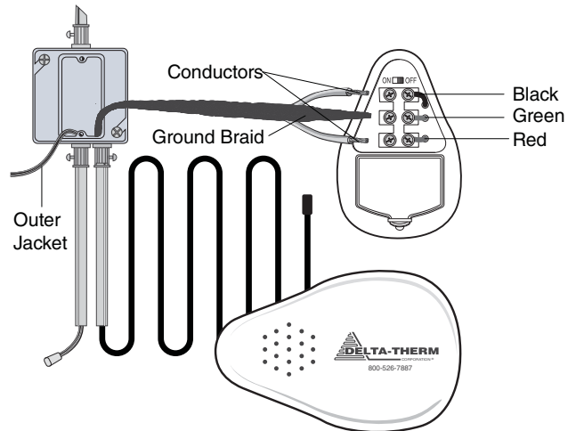
Detail 2. Connecting the floor warming cable to the back of the FloorWarner.
