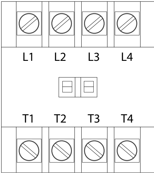
Detail 1. DT-X40A Contactor.
