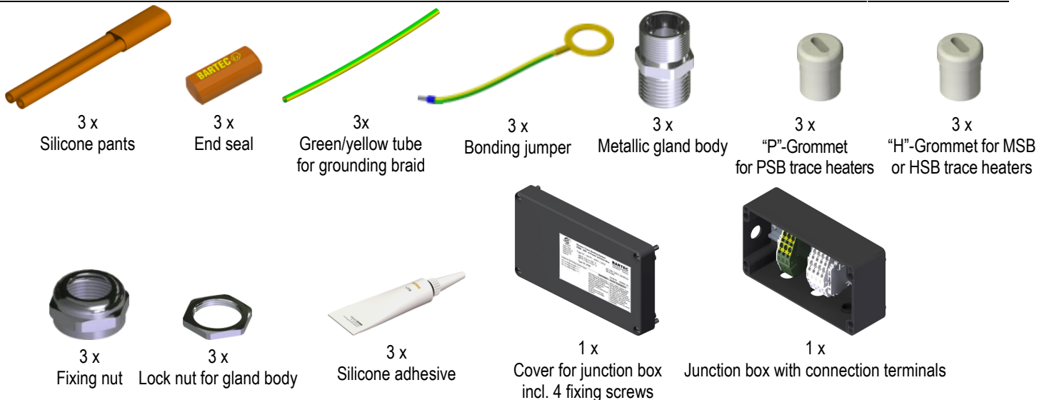
PBM-300-A Multiple entry power junction box
